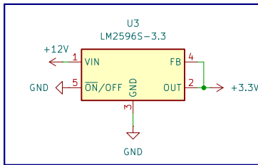
Buck converter
